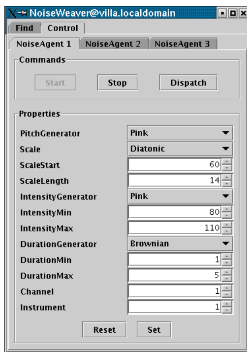
Figure 4: The NoiseWeaver GUI
